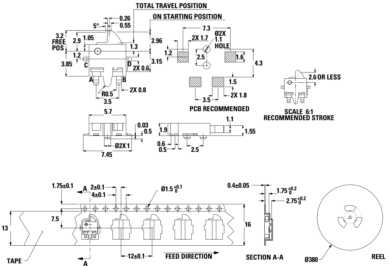
Dimensions (mm)
